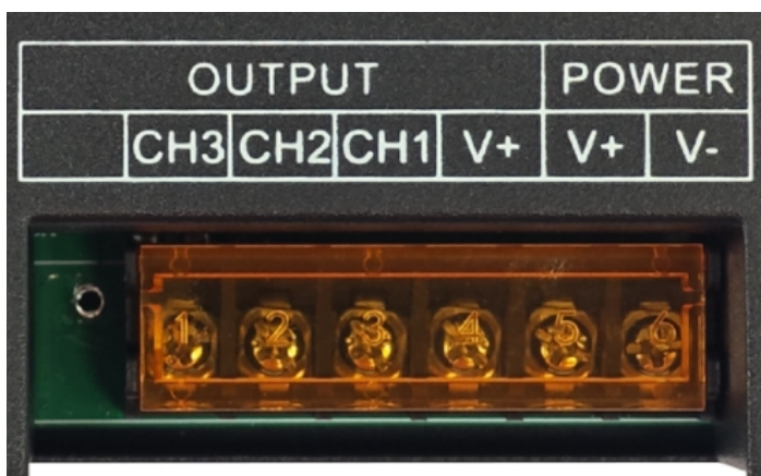
Power and Load interface: Use iron terminals with screws
