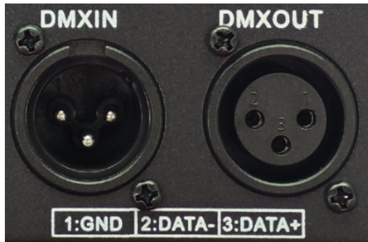
DMX Input/output interface:
