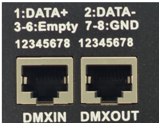
DMX Input/output interface: RJ45 Port
