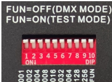
Address code and set feature service interface:
